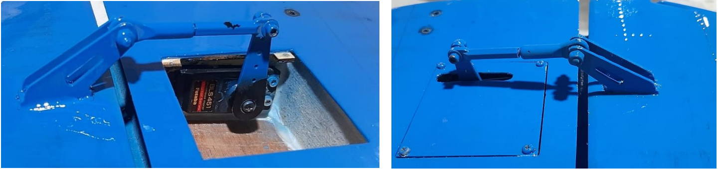
Above: elevators servos, servo arms and horns position with linkage.
