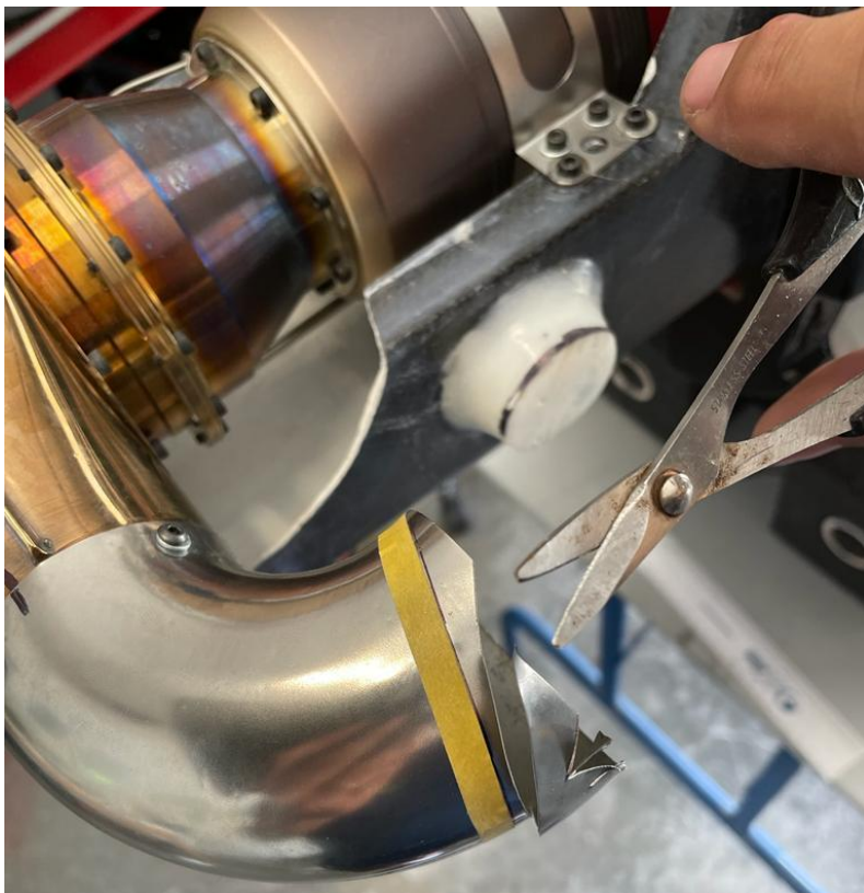
Above: exhausts cutting for realistic and scale appearance.
