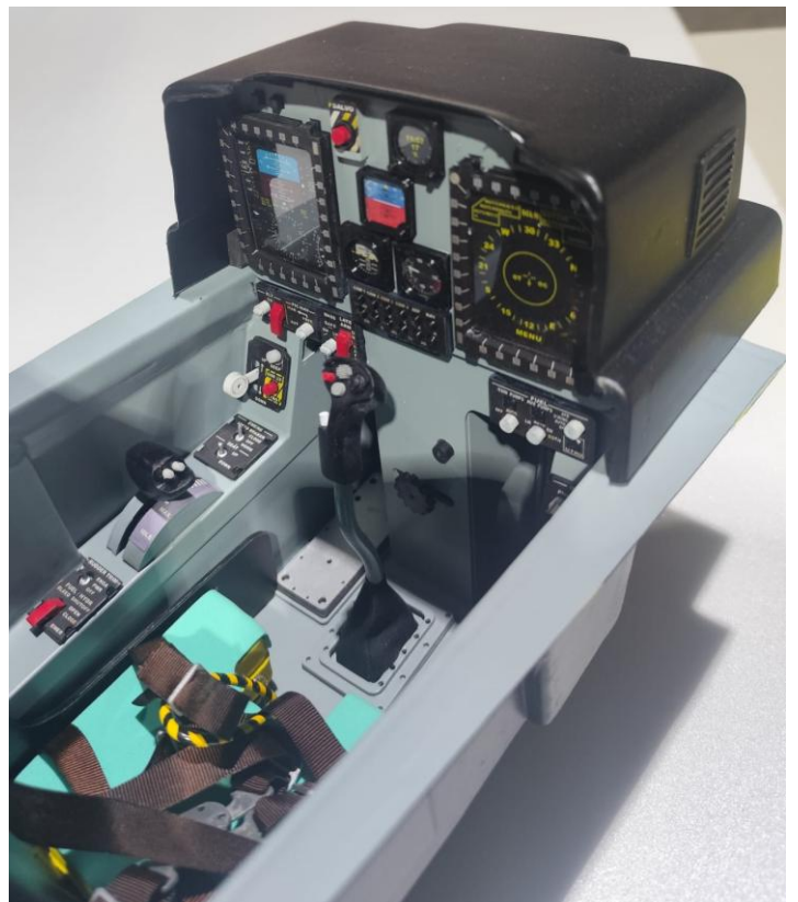
Above: rear cockpit details with panels, buttons and controls.
